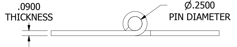
TYPE "L" LEFT HAND SLIP JOINT HINGE
