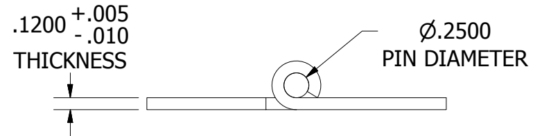
TYPE "R" RIGHT HAND SLIP JOINT HINGE
