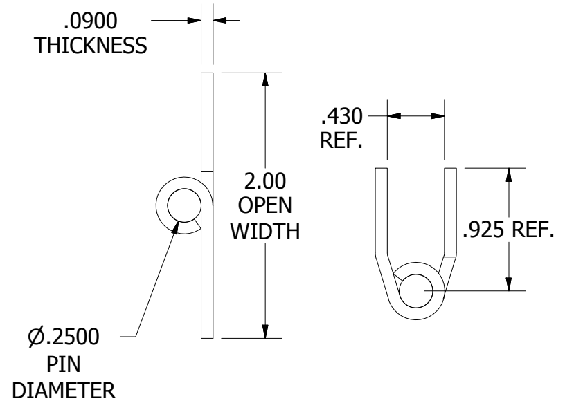
AFTER OFFSET (CLOSED POSITION)
