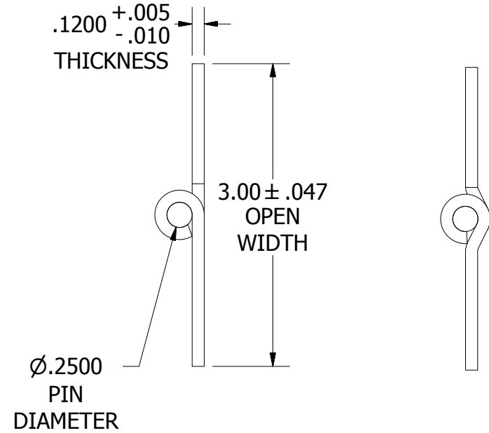
AFTER SWAGE
