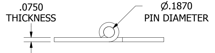
TYPE "L" LEFT HAND SLIP JOINT HINGE
