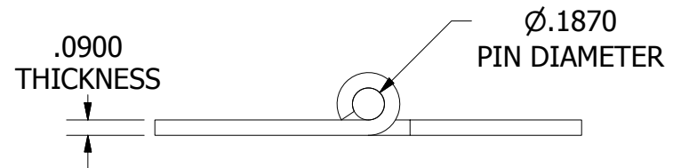
TYPE "L" LEFT HAND SLIP JOINT HINGE
