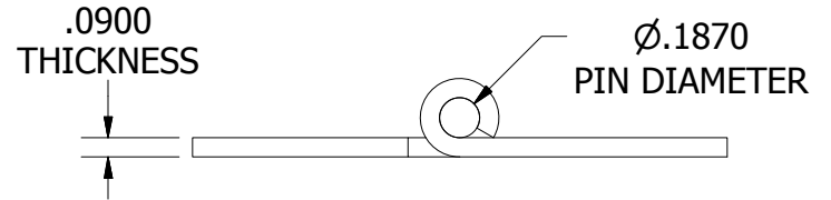
TYPE "R" RIGHT HAND SLIP JOINT HINGE
