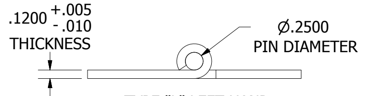
TYPE "L" LEFT HAND SLIP JOINT HINGE
