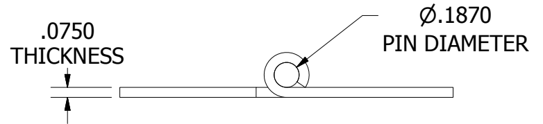
TYPE "R" RIGHT HAND SLIP JOINT HINGE
