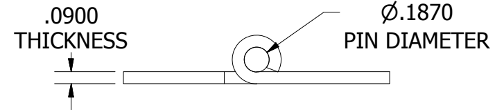
TYPE "R" RIGHT HAND SLIP JOINT HINGE
